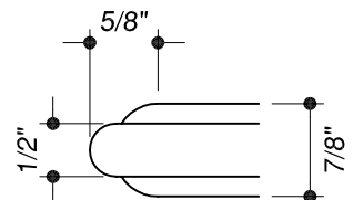
Neck Mold
