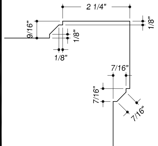
Recessed Panel Detail
