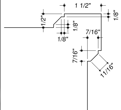
Recessed Panel Detail
